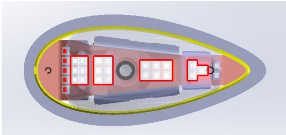
Figure 2: Strobe LEDs
