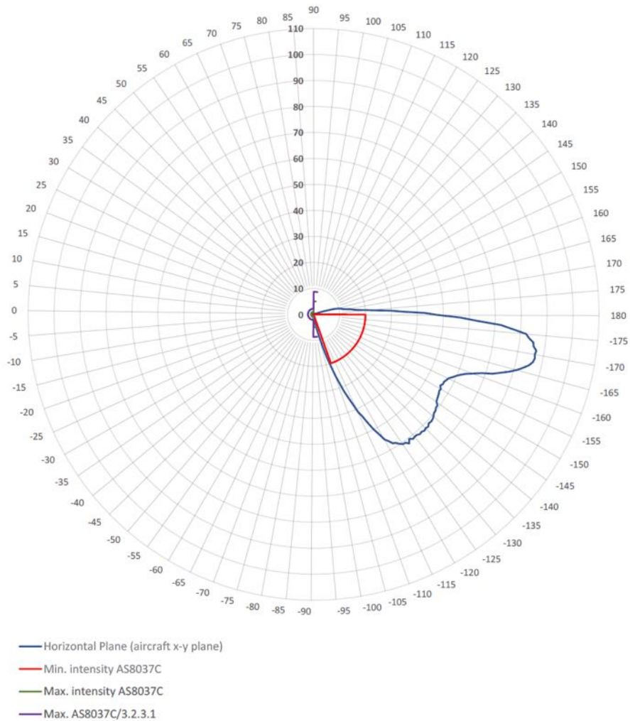
Aircraft Horizontal Plane, "0" direction is HOVO FWD. Full range, cd
